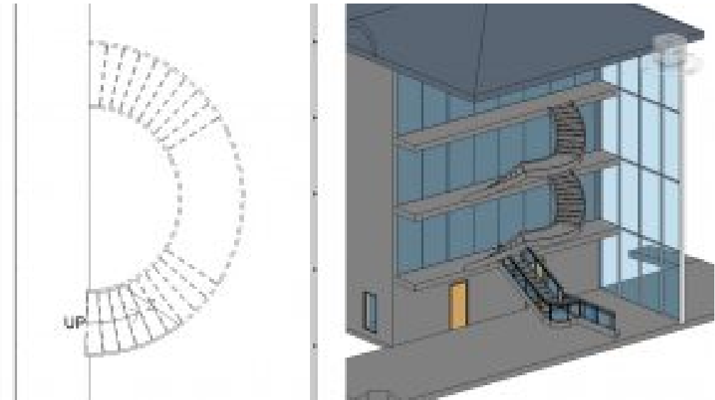
Figure 4.7 Spiral stair in plan view and in 3D view
