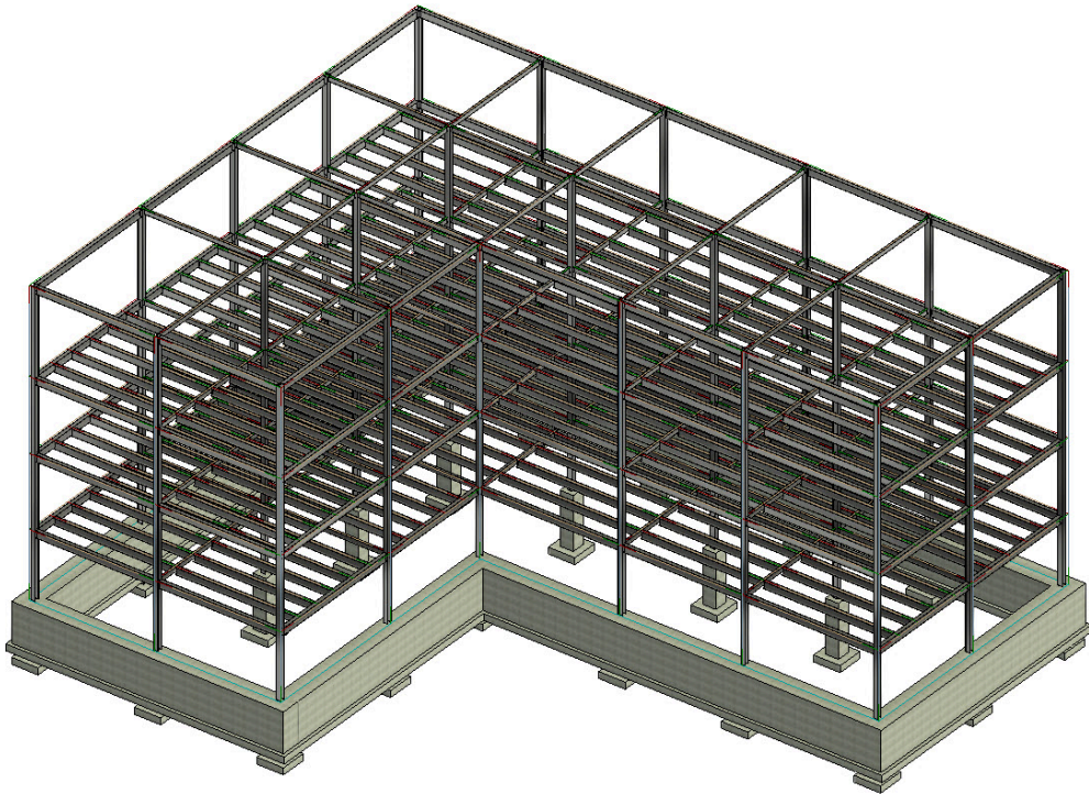
Figure 16.14 Beam System placed on level 3 and 4, shown in 3D view
