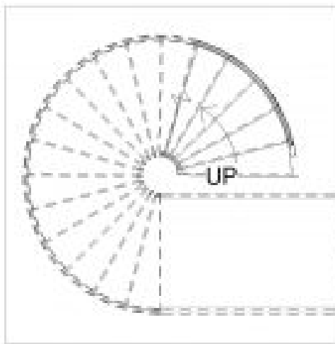
Figure 4.6 Spiral stair in plan view and in 3D view
