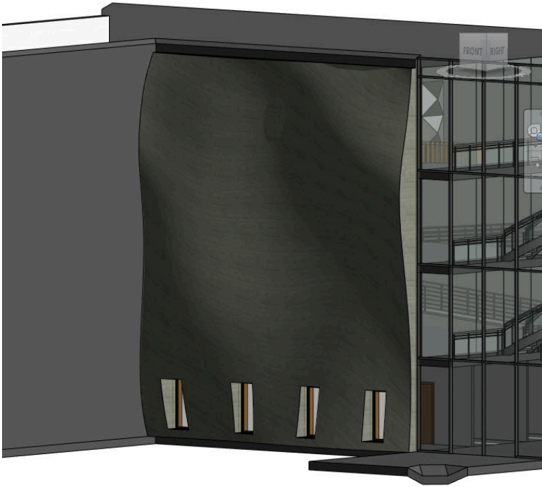
Figure 7.19 Completed Curvilinear façade shown in 3D view
